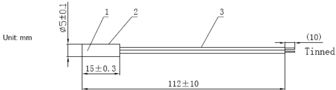
Temperature Sensor: 0.6" stainless steel probe temp sensor, 10Kthermistor, standard Curve 3
